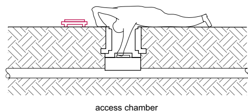
access chamber
