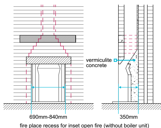
fire place recess for inset open fire (without boiler unit)
