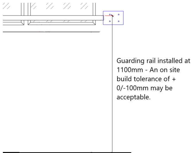
Figure 2: Example of how build tolerance may be shown on plan for overheating windows also used for means of escape.
