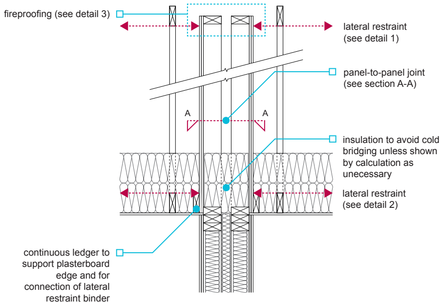
TYPE TWO Single leaf spandrel panel supported on a timber framed party wall
