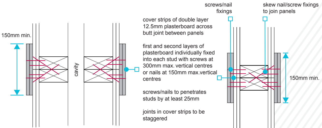
Section-view A-A of joint in spandrel panel
