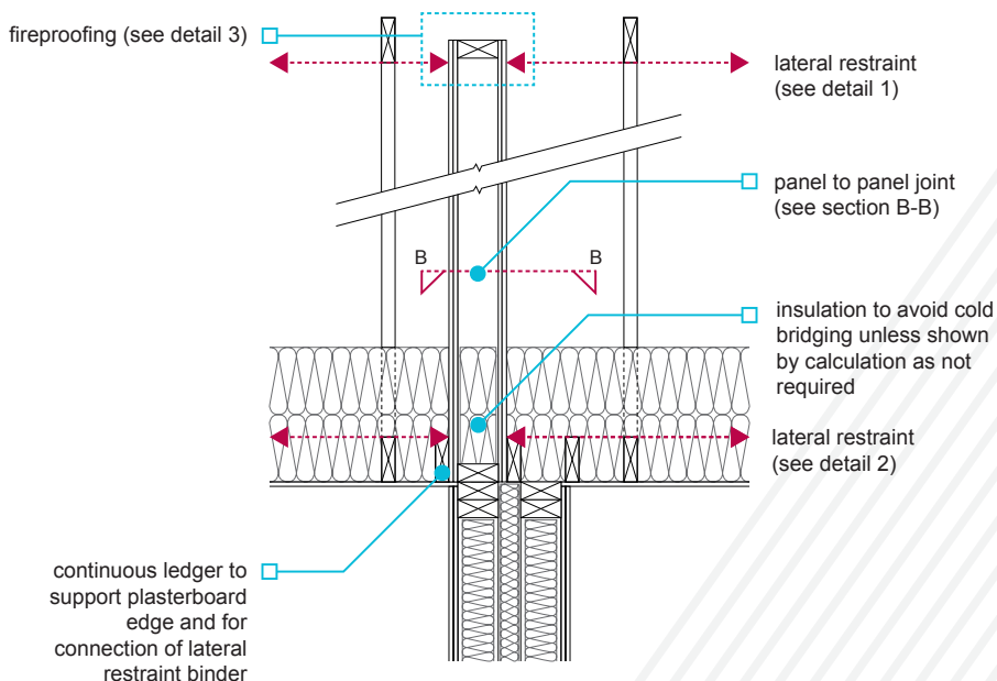
TYPE TWO Single leaf spandrel panel supported on a timber framed party wall
