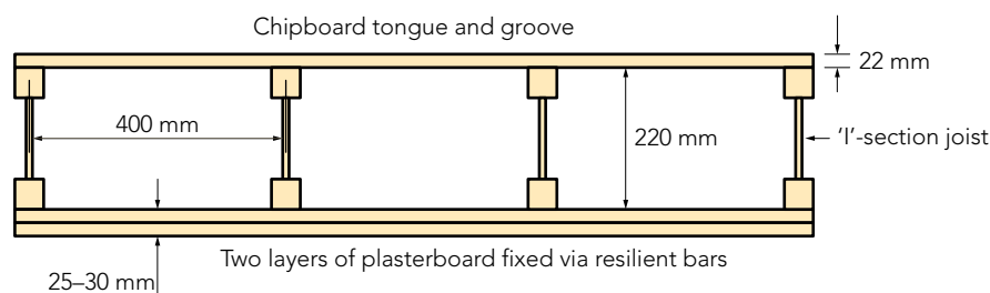
Figure 29 Typical section through floor.
