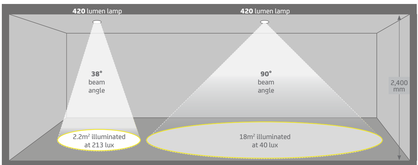
Figure 7 Importance of beam angle. These two low-energy lamps (with the same lumen output) generate a quite different illumination level (lux) and light coverage area (m 2 ) at floor level.
