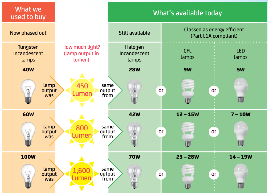
Figure 2 Compared with tungsten incandescent light bulbs, modern lamps, particularly CFLs and LEDs, require a fraction of the power to generate an equivalent level of light.
