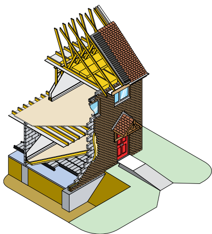
Typical masonry cavity construction
