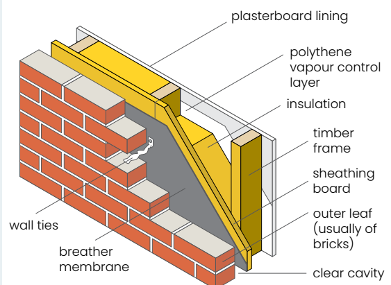
Timber frame external wall construction
