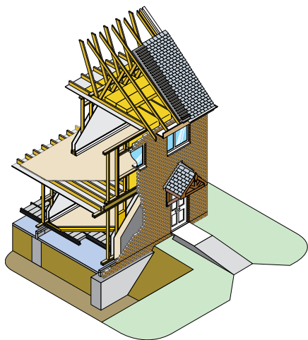
Typical timber frame construction
