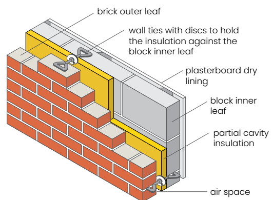
Cavity partially filled with insulation
